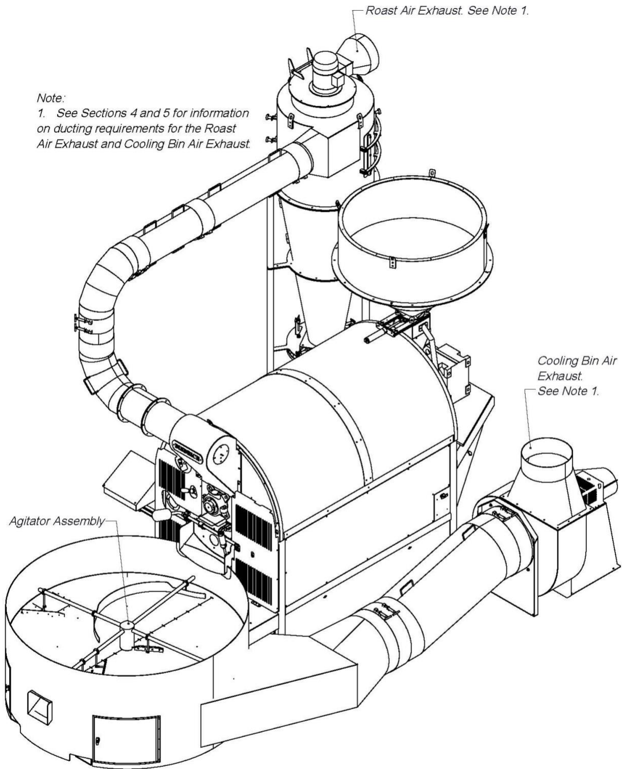
Front Right - Isometric View
