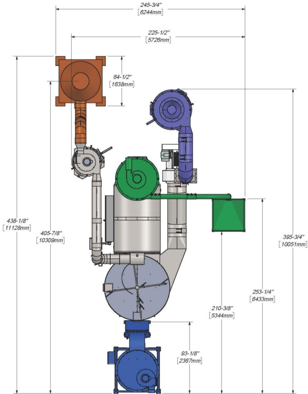
Top View - Full Roasting System
